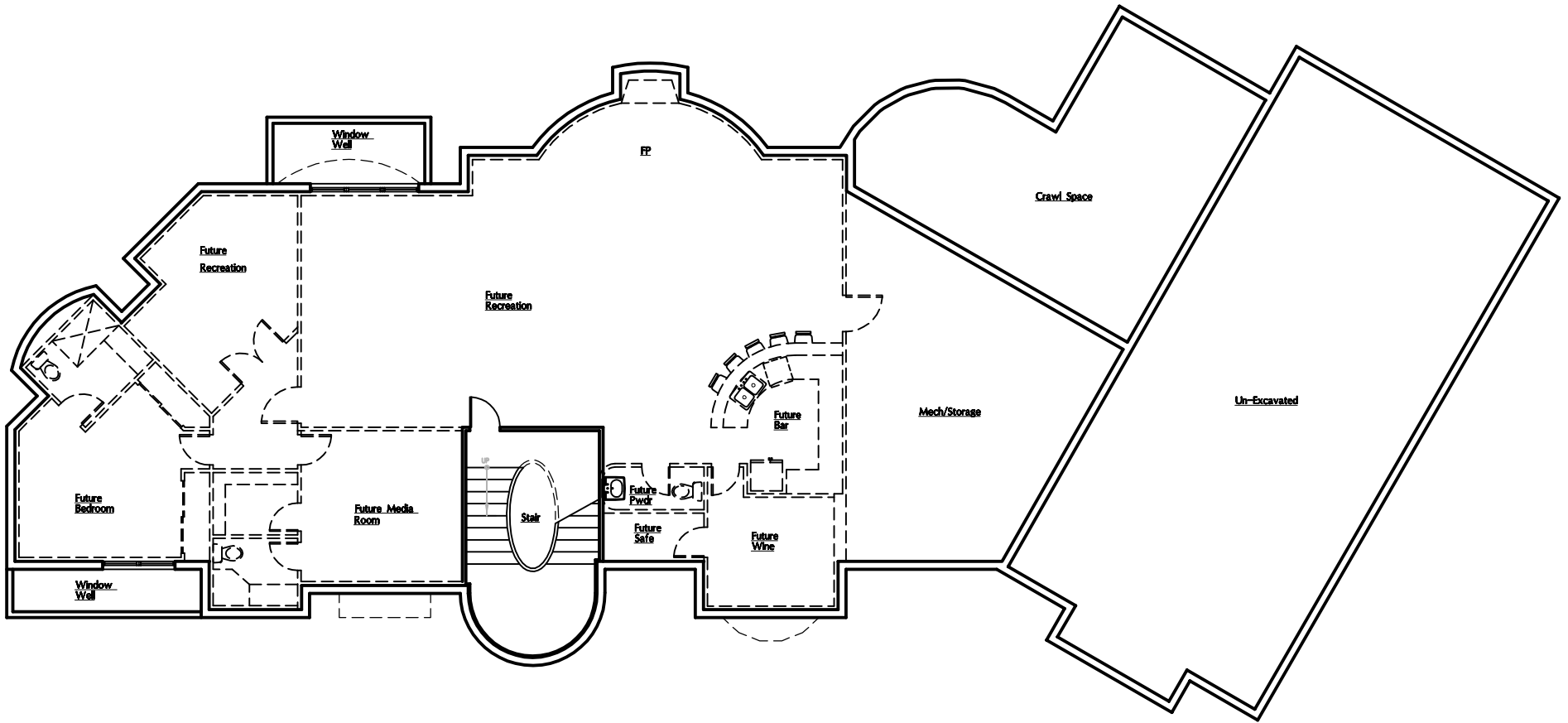
Basement Floor Plan Scale: 1/4" = 1'-0"
